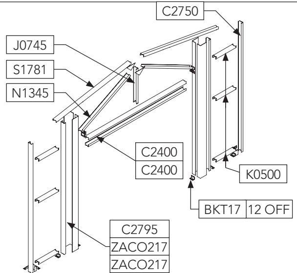
Side mullion assembly
